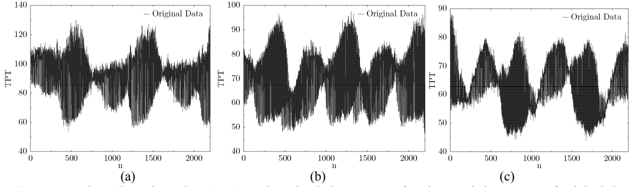
Figure 3: Excerpt plots (throughput time (TPT) against simulation steps n for characteristic patterns of original data retrieved from the simulation for different values of L (evaporation parameter). (a) pattern A with L = 50 , (b) pattern B with L = 150 , and (c) pattern C with L = 250 . Note: the plots reflect the first 2200 samples of data points from each dataset after stripping data from initial attack times
