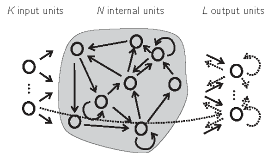
Figure 1: ESN architecture: an ESN has three layers. Solid arrows indicate mandatory types of connections, dashed arrows are optional connections. Figure reproduced and adapted from Jaeger (2001)
