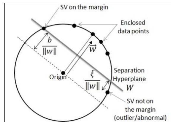
Figure 4: One-Class Support Vector Machine (Lecomte et al. 2011)
