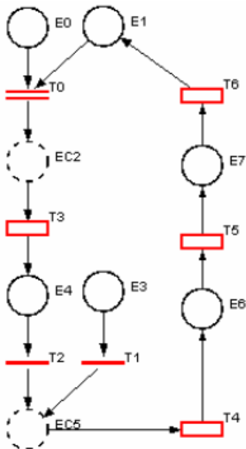
Figure 3. CCPN obtained from four ECA rules.
